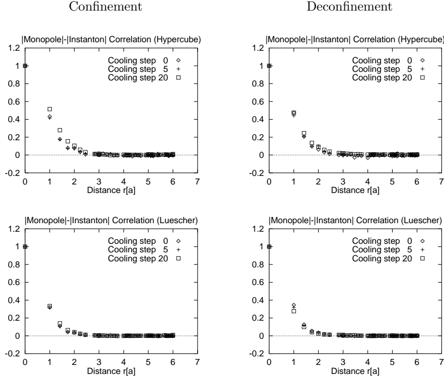
Figure 2. Correlation functions between the monopole density and the absolute value of the topological charge density for the hypercube definition and the Lüscher definition in the confinement (l.h.s.) and the deconfinement phase (r.h.s.) for 0, 5, 20 cooling steps. For both definitions the monopole-instanton correlation functions are almost invariant under cooling and extend over approximately two lattice spacings. The correlation functions hardly change across the phase transition.
